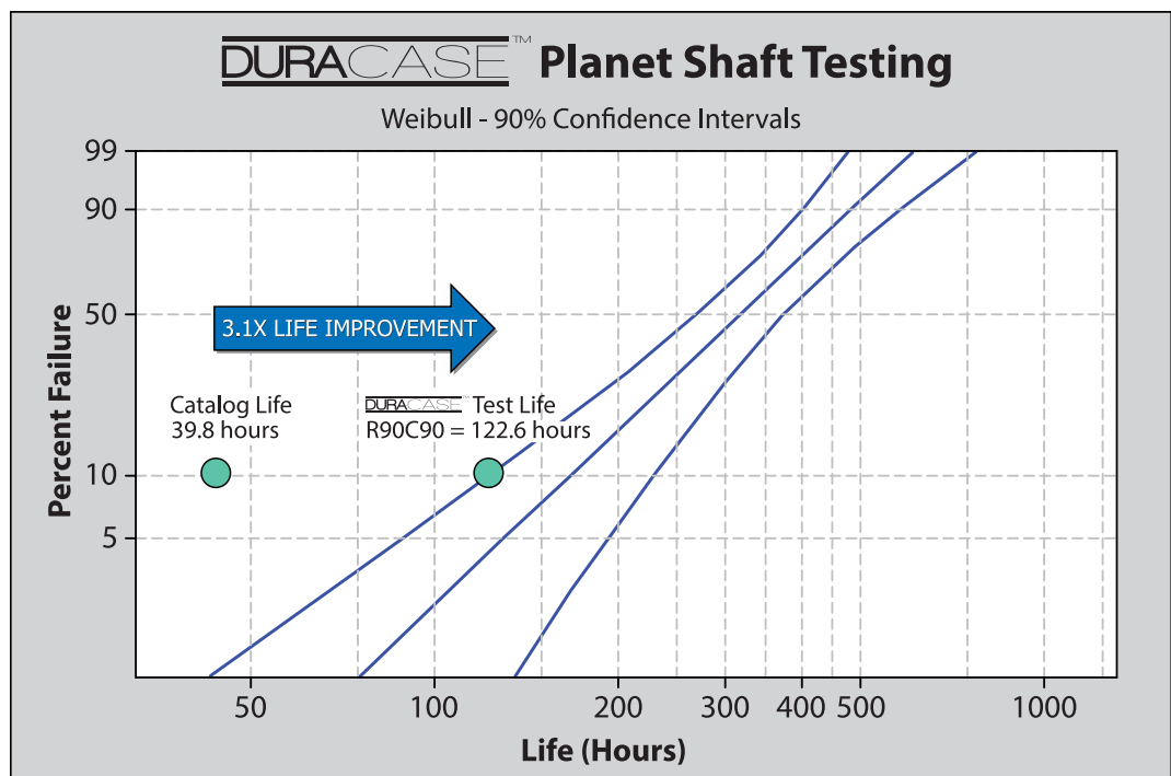
The graph above displays a 3.1 times life improvement compared to industry standard catalog life calculation.
