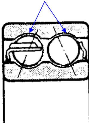
Radial Internal Clearance
